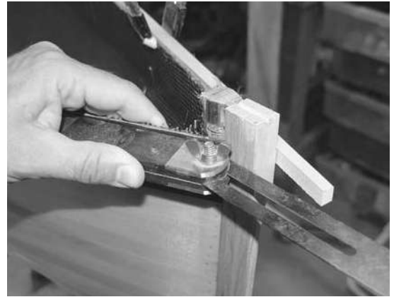
Figure 12-30. I extended the outwales onto the stem by tapering the ends. Use a bevel gauge to transfer the angle to the outwales.
