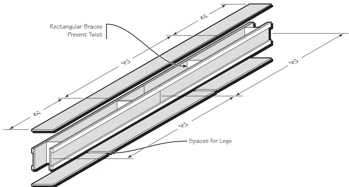
Figure 5-17. You don't want all the joints on the box beam to line up. For a 16-foot-long beam, cut two of the top and bottom pieces in half and put the half pieces at the end with the long piece in the middle. With a large external box beam a couple of braces inside the beam help prevent twist. If you leave some open slots in the bottom, you can insert legs into the beam instead of using sawhorses.
