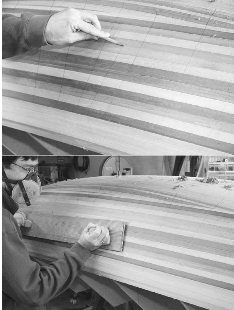
Figure 11-17. To get a fair, consistent surface you want to sand everything to approximately the same degree. You can provide sanding guides by scribbling on the surface with a soft pencil. Do not press hard, and use the side of the pencil point so you don't create grooves in the wood.
