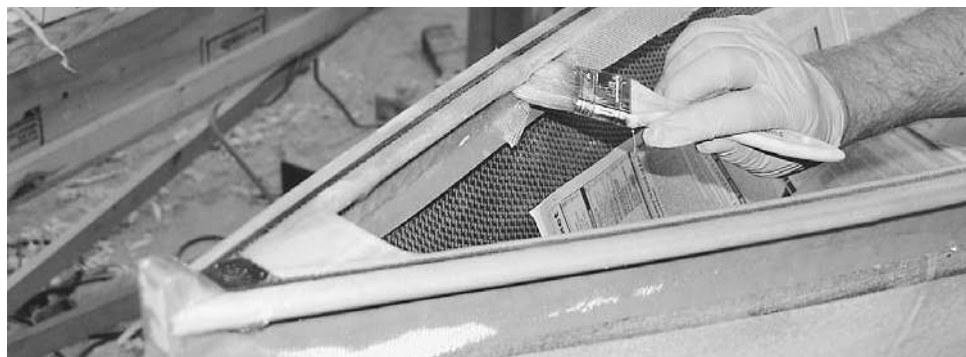
Figure 12-35. The gunwale will be covered with 3-inch-wide bias-cut strips of fiberglass. Run masking tape about \frac{1}{4} inch below the bottom of the gunwale, then lay out the glass strips.
