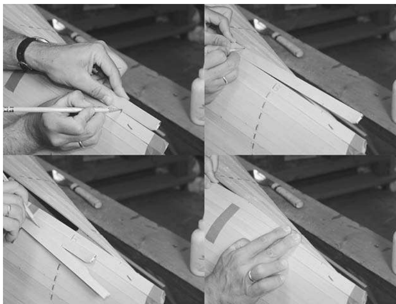
Figure 12-18. Now it is time to close up the bottom. Fit strips into the bottom gap by marking both the length and where the upper edge of the strip crosses the gap. Connect these two points and then trim to that line.
