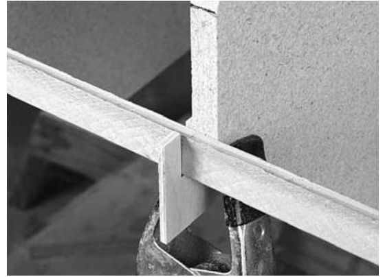
Figure 6-9. Getting the first strip aligned on the forms to create a smooth, fair curve may require a little finagling. Use some U-shaped jigs to temporarily hold the strip in place while checking the alignment. When you have it right, secure the strip in place with a staple or other fastener.
