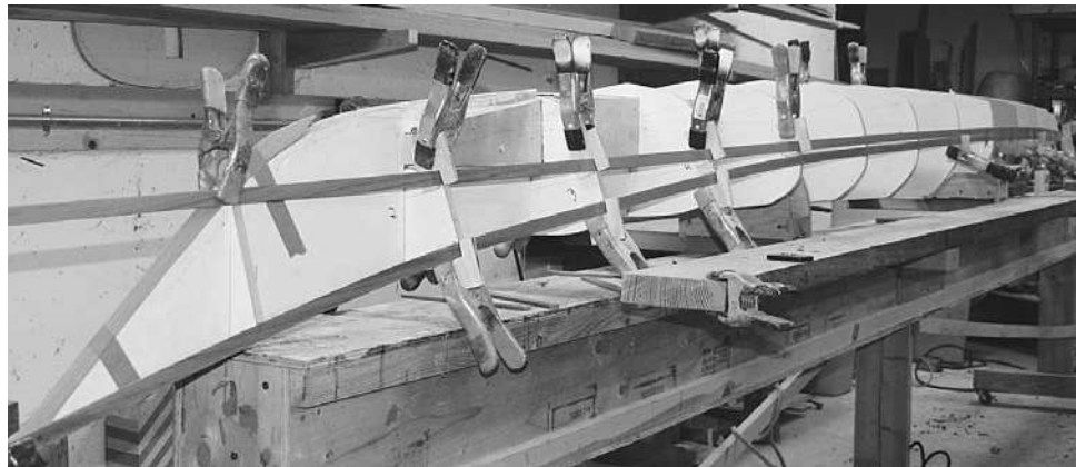
Figure 13-20. The first strip follows the sheerline (bottom strip), and the second follows a more straight line. This second strip actually follows a diagonal line that is parallel to the run of the chine. In this way, by the time you strip up as far as the chine, the strips will approximately follow the chine so the joint with the next strip will be easier than it would be if it went in some other obscure direction.
