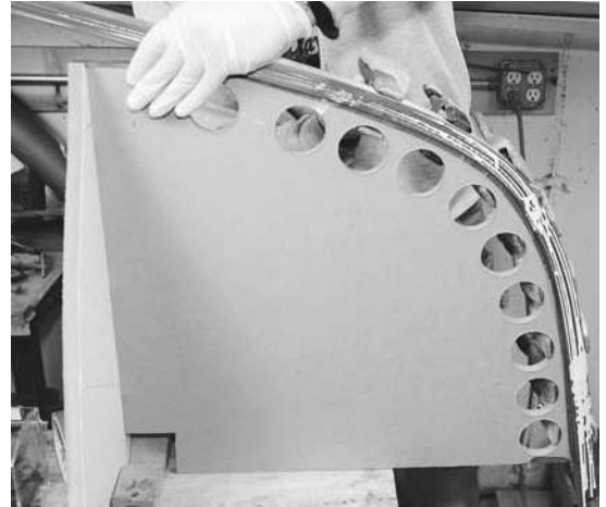
Figure 5-27. For boats where the stem takes a sharp bend, a bent inner stem works better. This can be laminated or steam bent. With thin enough laminations, the stem will bend easily around the form. The topmost lamination is backed up with fiberglass-reinforced tape to help protect against splitting. This helps the wood bend around a tighter radius with less chance of breaking.
