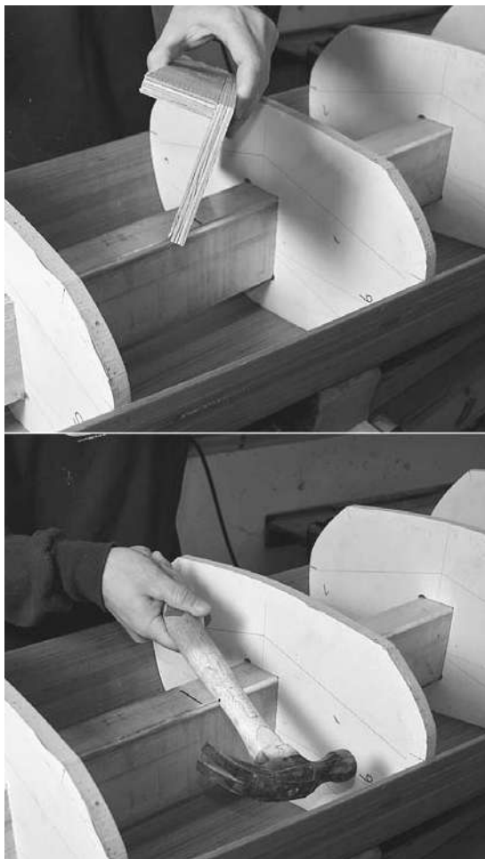
Figure 13-28. When the hull is completely stripped, you can flip over the boat onto some foam cradles or slings. Since it will be harder to do after the deck has been installed, I knock the forms free now. Remove the wedges from the middle spacer and lift out the other spacers. Hit the forms with a hammer to break the hot-melt glue holding on the strips. Make sure you break free the end forms as well. When they are all free (so you will eventually be able to remove the hull), insert the spacers back in place.
